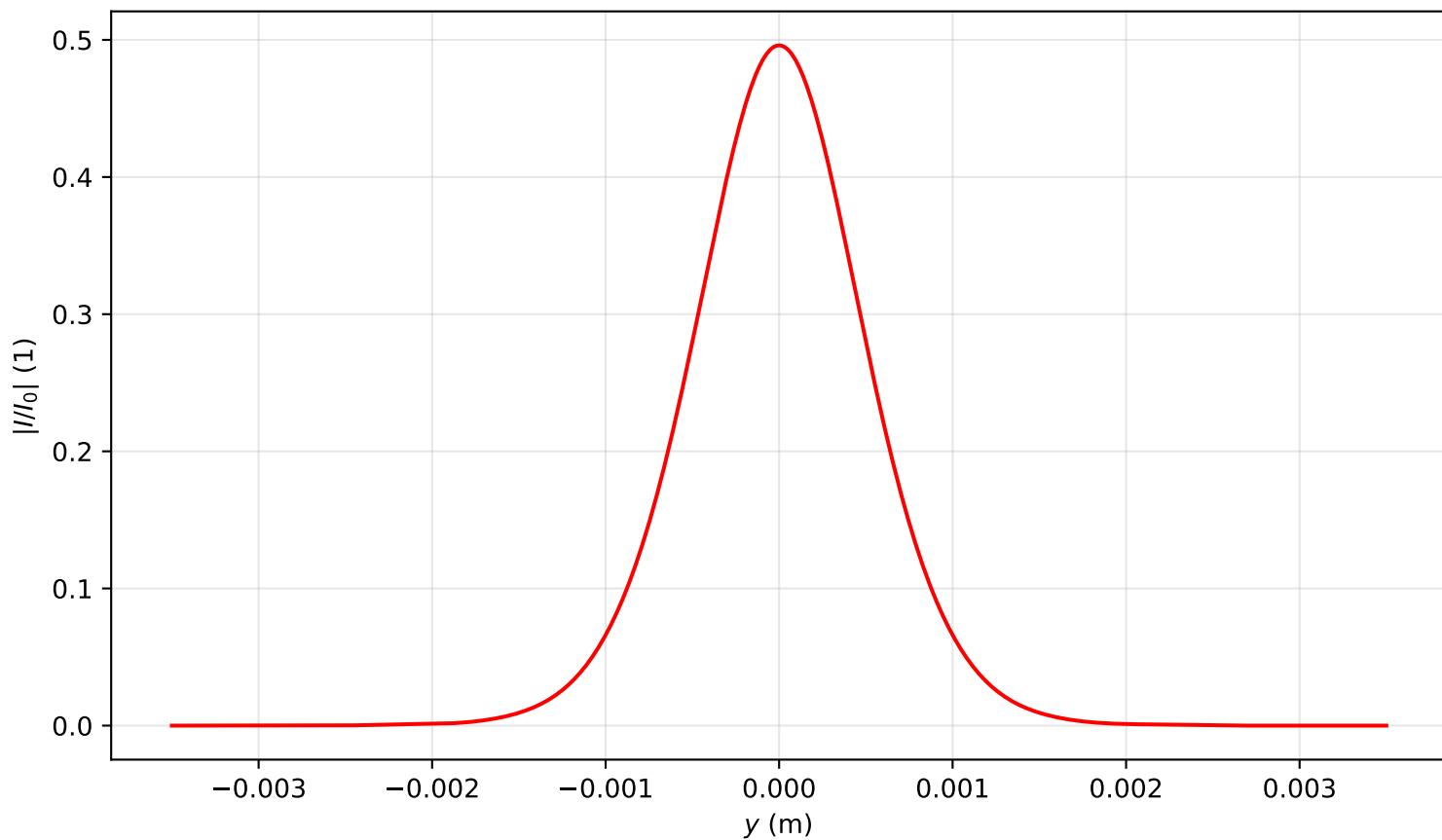
Intensity profile I(x = 0, y, z = 3.344)/I_0 , P_{in}=0.5P_{cr} , artificial time
